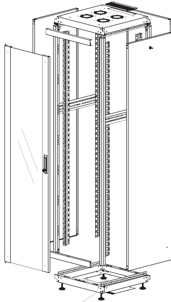
Exploded view
